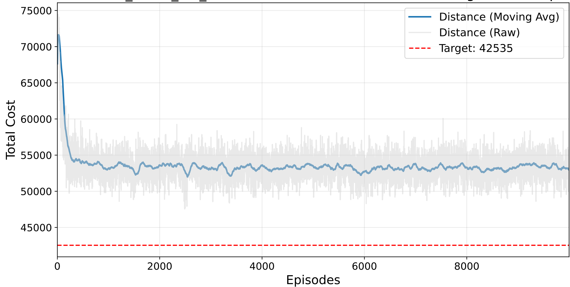
Final NO_MASK_NO_BAYESIAN Masked AutoRL-SOP Training - ft70.3.sop
